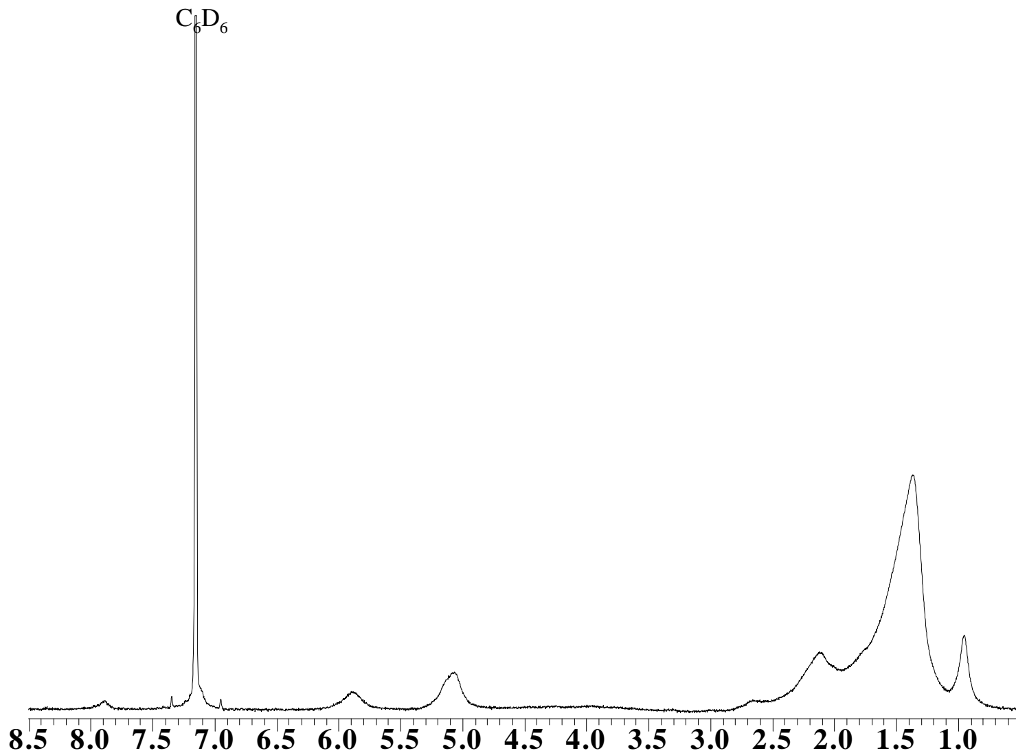
Figure S3: ^1\text{H-NMR} spectrum of photolyzed MUP-C 12 MPC that has been washed to remove liberated acetophenone in benzene- d_6
