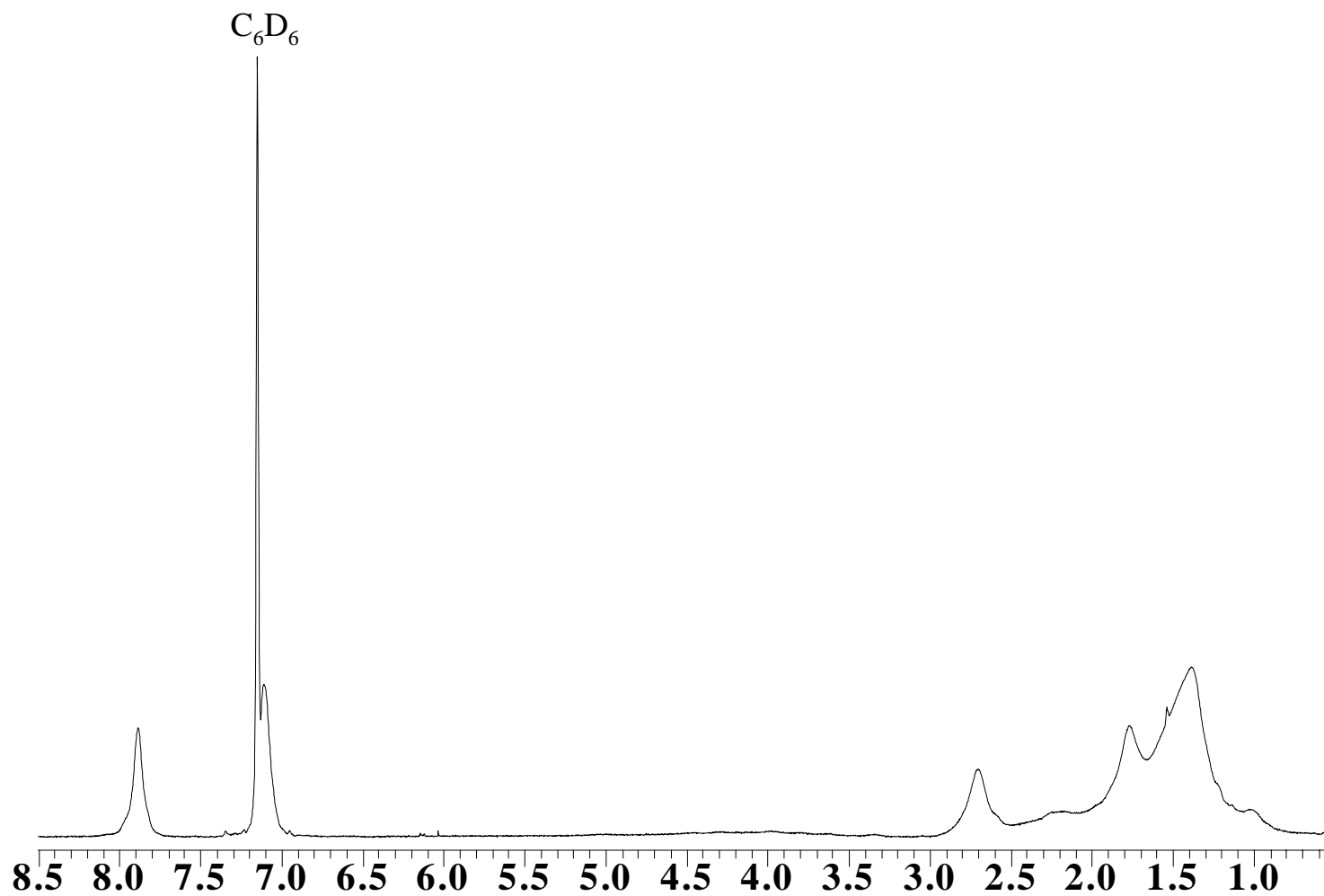
Figure S2: ^1\text{H-NMR} spectrum of MUP-C 6 MPC before photolysis in benzene- d_6
