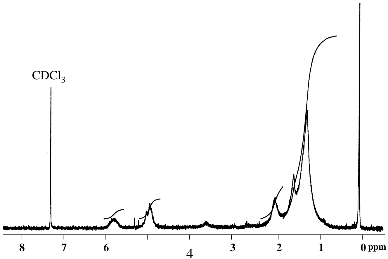
Figure S5: ^1\text{H-NMR} spectrum of 11-mercaptoundecene MPC in \text{CDCl}_3 .
