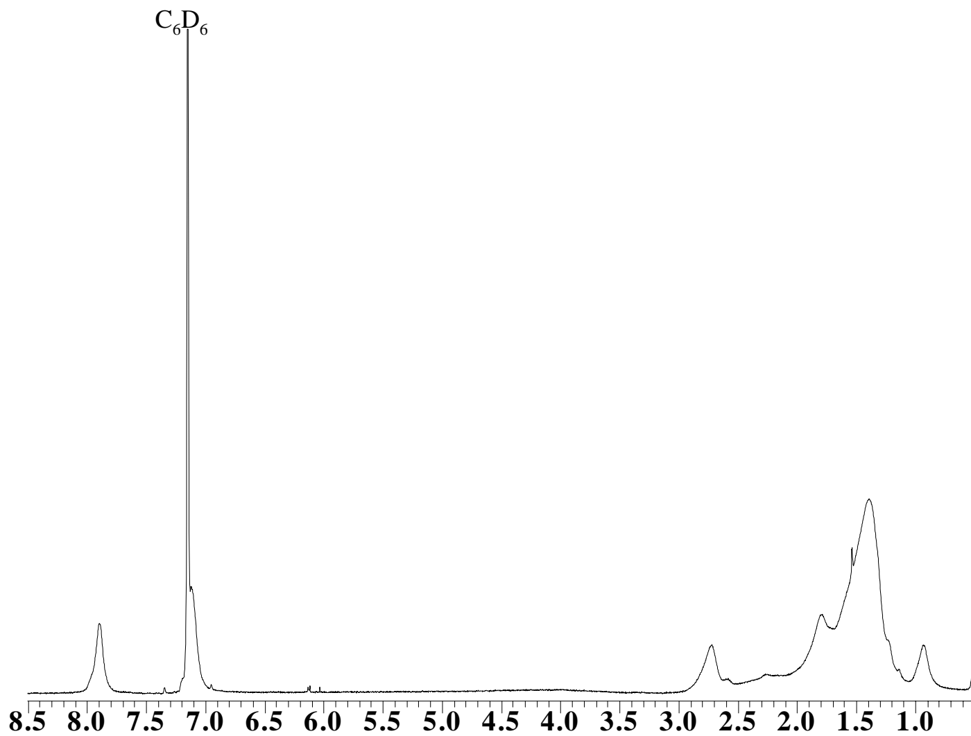
Figure S1: ^1\text{H-NMR} spectrum of MUP-C 12 MPC before photolysis in benzene- d_6 . Same as Figure 1a.
