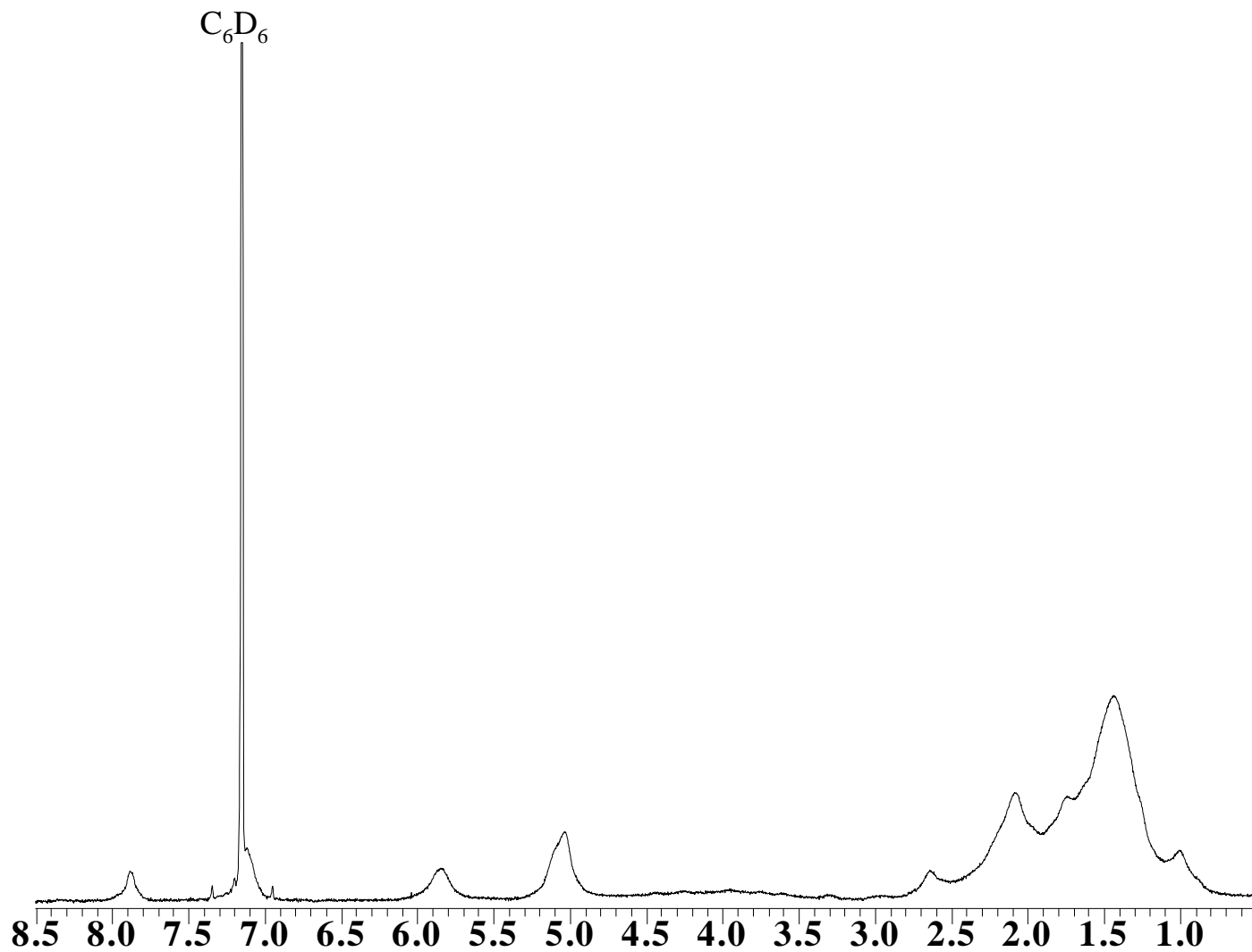
Figure S4: ^1\text{H-NMR} spectrum of photolyzed MUP-C 6 MPC that has been washed to remove liberated acetophenone in benzene- d_6
